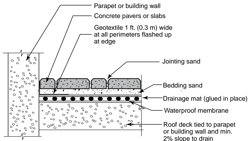
Figure 10. Detail showing geotextile at all edges of sand and aggregate bedding courses for a pedestrian application.
