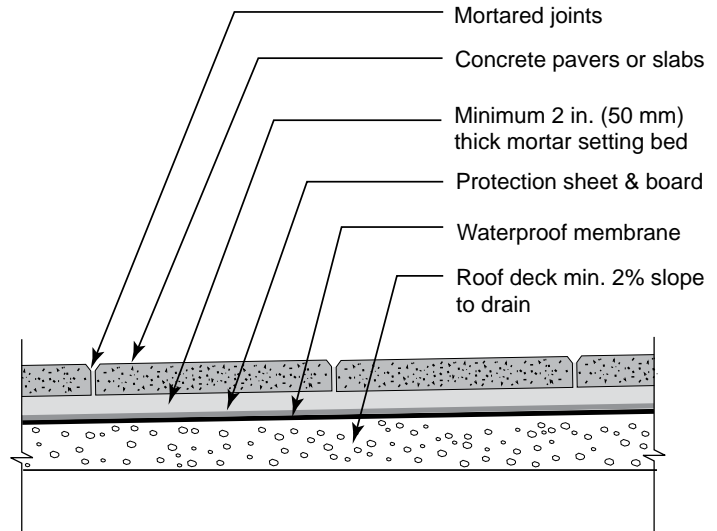
Figure 9. Mortar bed under paving units
