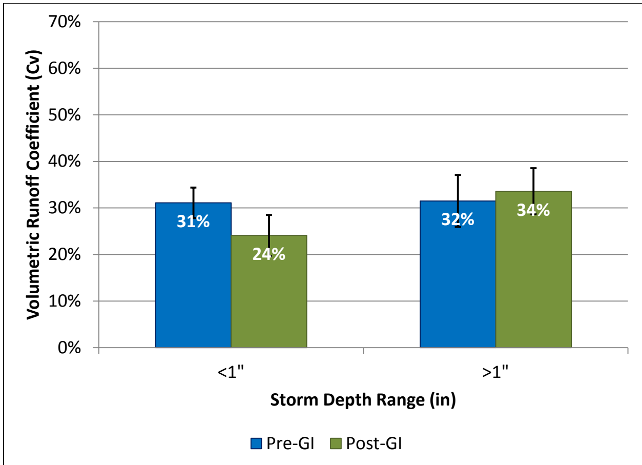
Figure 5-12: Average Volumetric Runoff Coefficient Based on Storm Depth with 95% Confidence Intervals Shown
