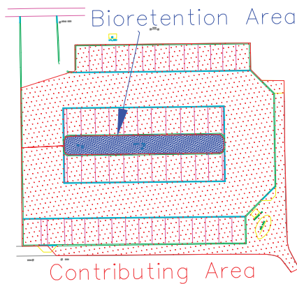
Figure 7.5.1: A post-construction survey provides an accurate measure of the drainage area and size of the practice to compare to the design plans. The survey can also show if there is any problem with stormwater flows bypassing the practice. (Source: CVC)
