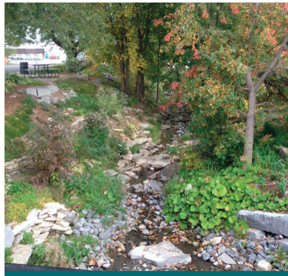
Figure 4.4.2: A buffer of natural vegetation has been established along this drainage channel. This beautifies the site and provides a stormwater filtration function. (Source: Fern Ridge Landscaping)
