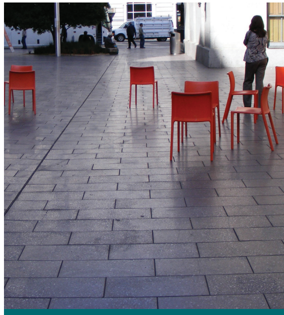
Figure 2.4.1: This urban parkette detains runoff and allows for infiltration through an underground chamber. The patio area is sloped towards the permeable joint running along the left of this photo. (Source: Aquafor Beech)
