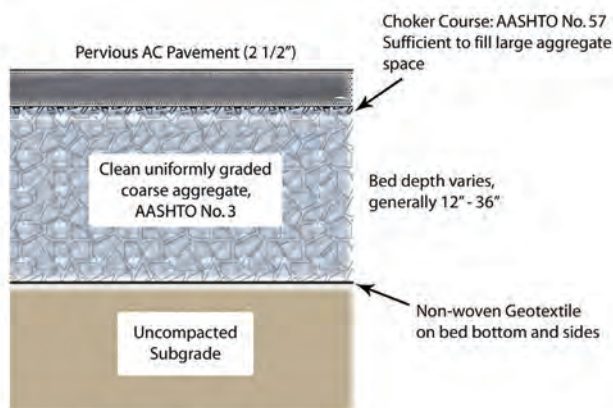
Example cross-section of porous pavement.
