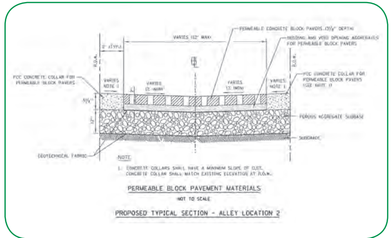
Permeable block profile
