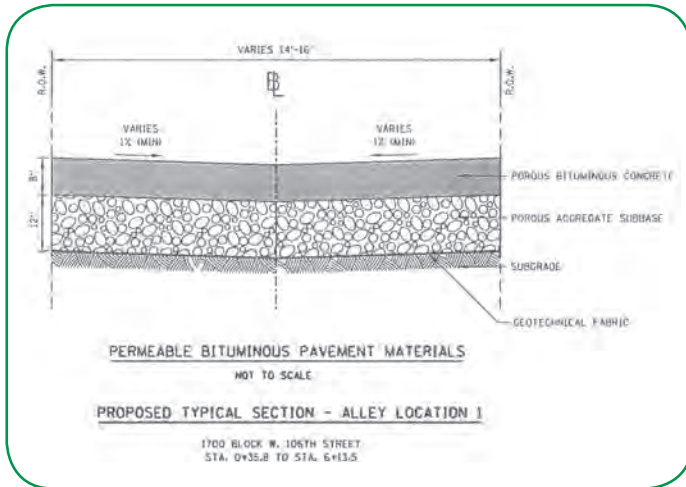
Permeable pavement profile
