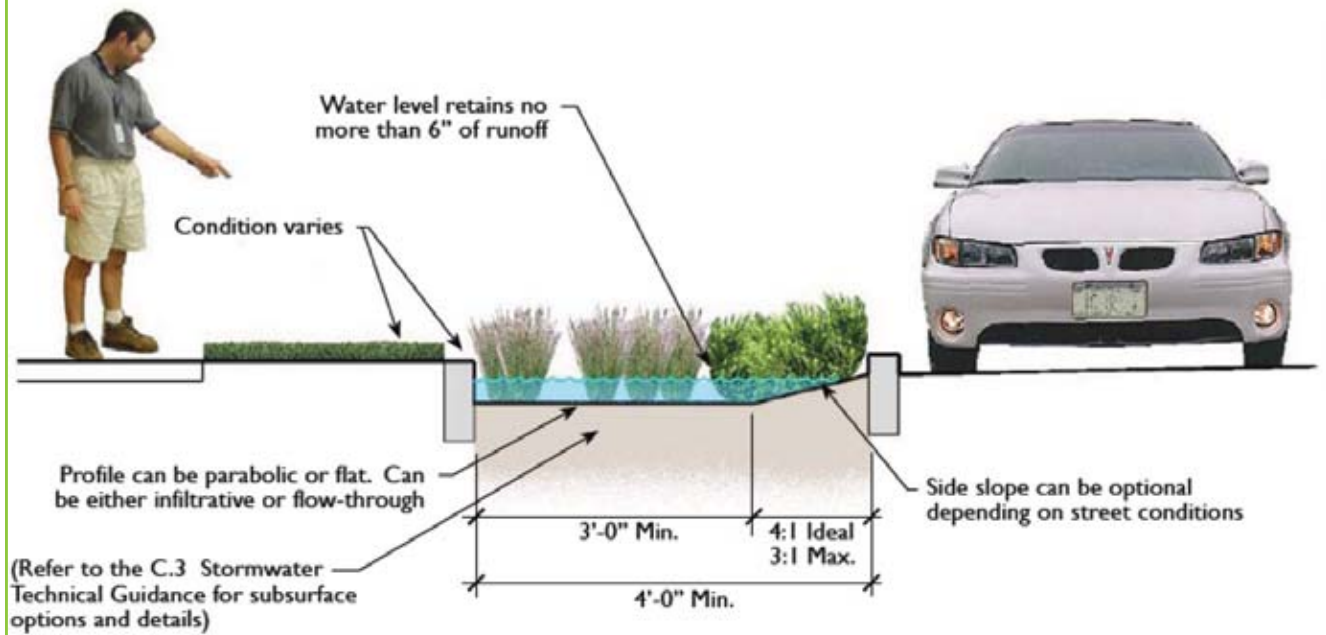
TYPICAL CURB EXTENSION PROFILE
